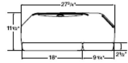
Split-pad Corner Platform U-B-488-25
