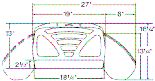
Banana Board Platform (assembly required*)
