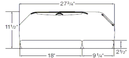
Split-Pad Corner Platform fits corner workstations:
