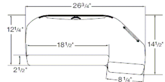
Reversible Corner Platform (assembly required*)
